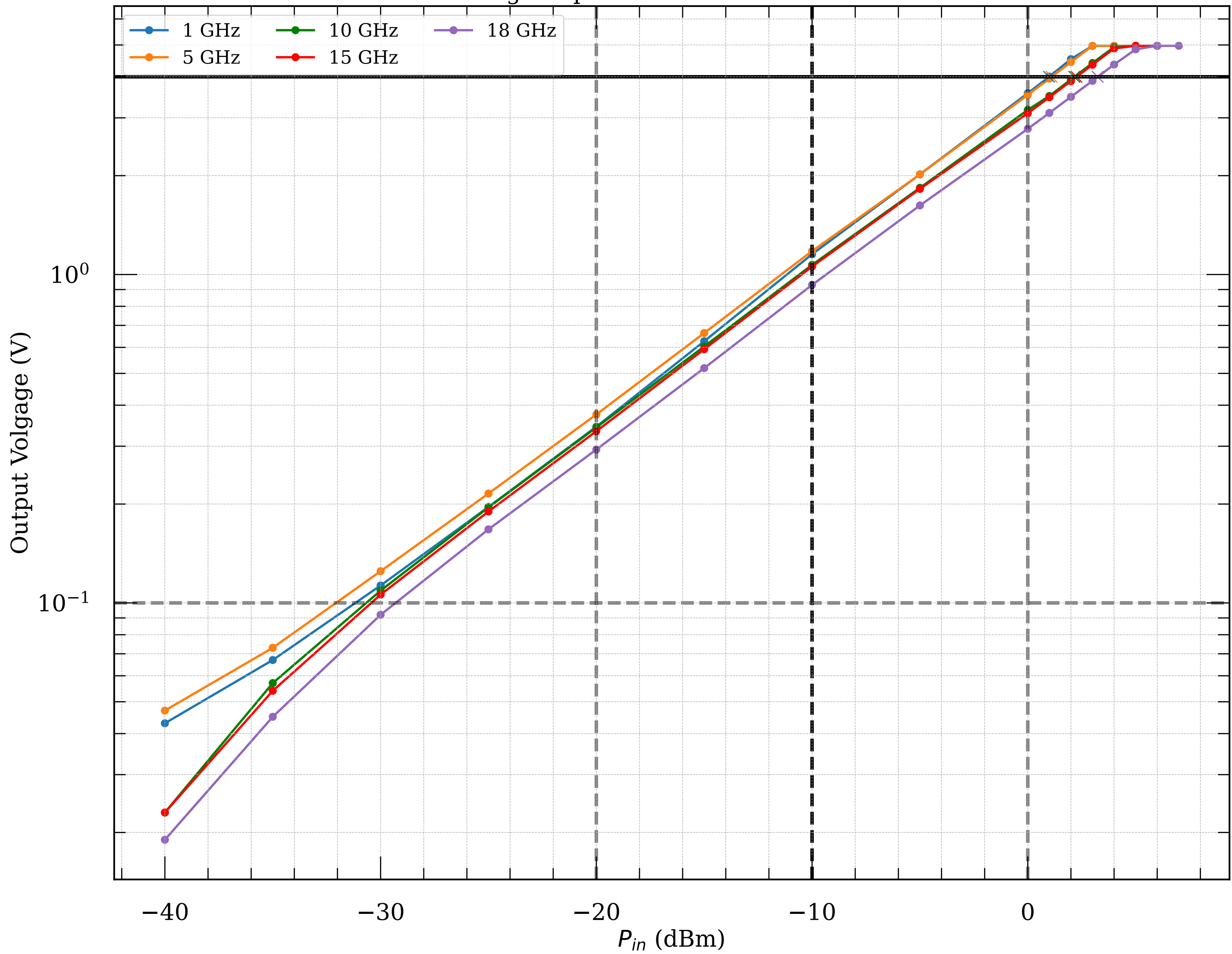
Measured voltage-to-power curve of detector module033v2
